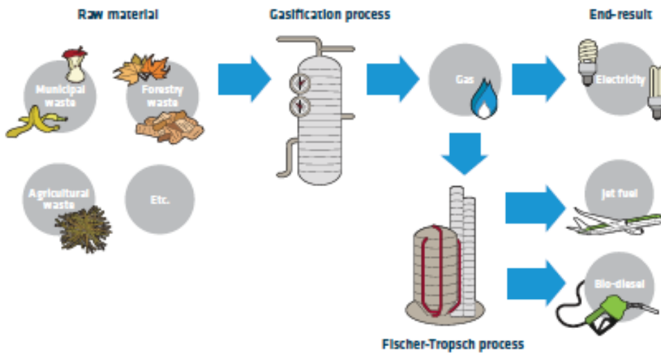
Figur 25 BTL-process
